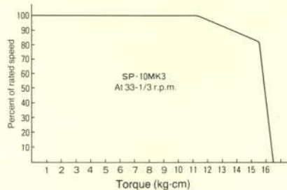
Load Characteristics
