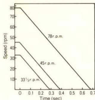
Braking Time
