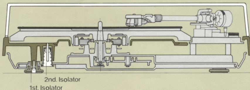
Cross section of SL-1301
