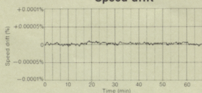
Speed drift
