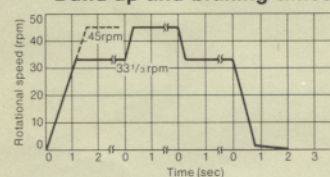
Build-up and braking times
