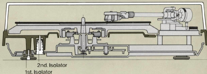
Cross section of SL-1301
