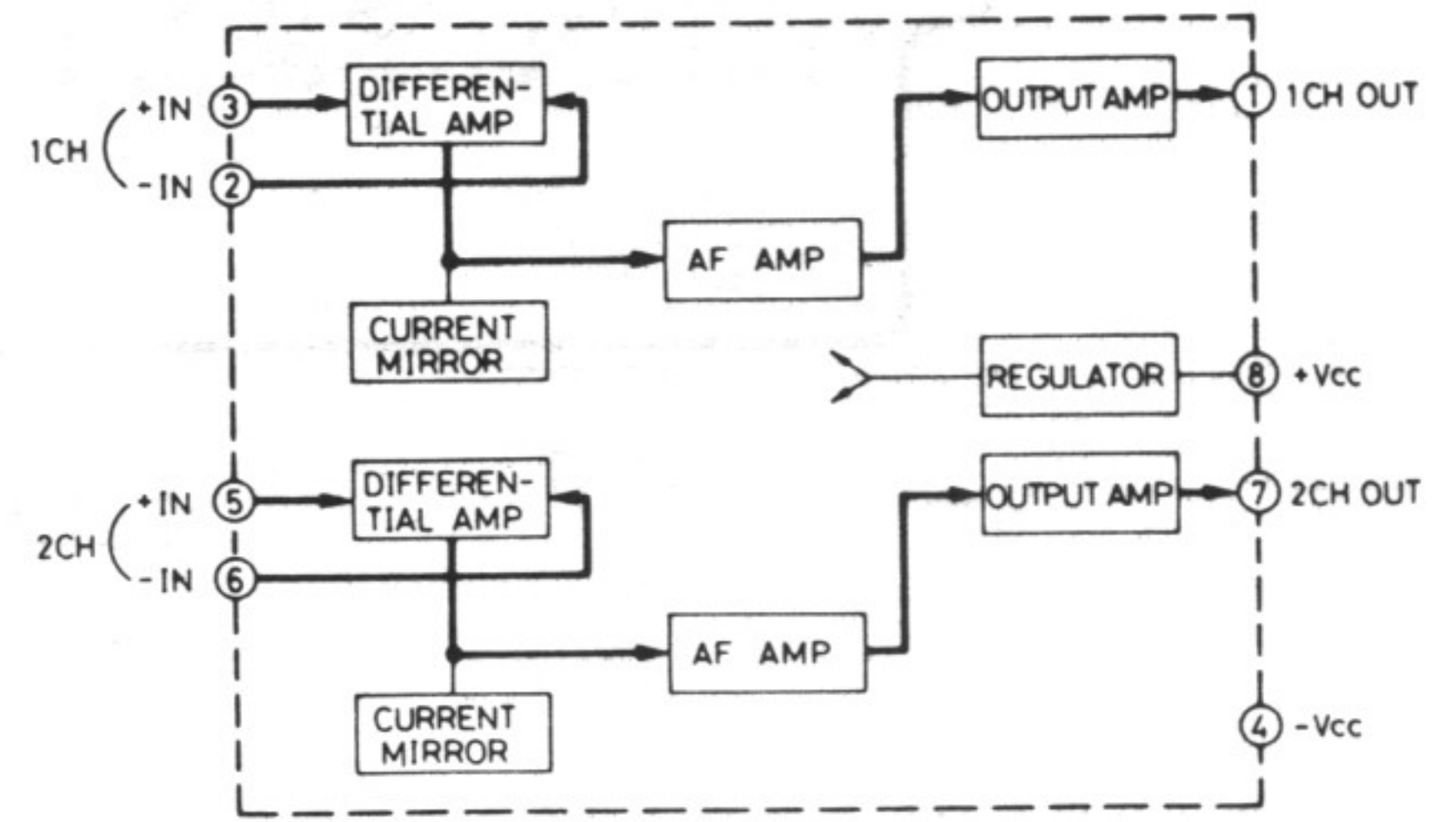
IC301 (SVIUPC4558C) DC Amplifier
