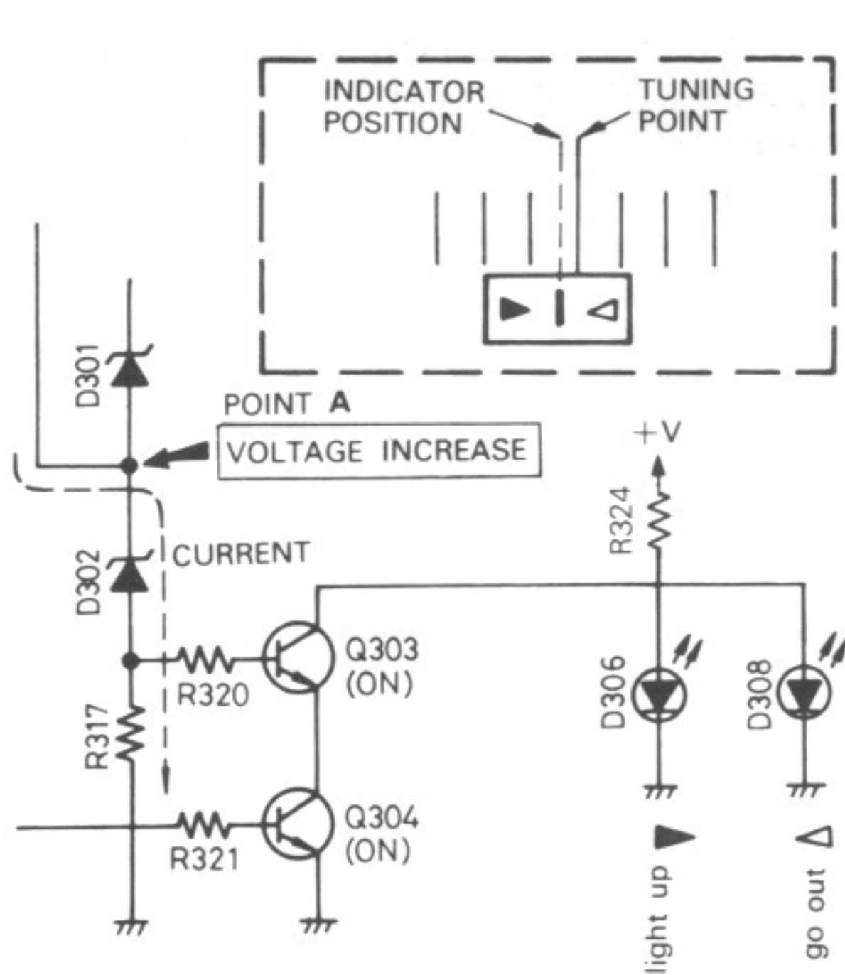
(Deviation to lower frequency) Fig. 9
