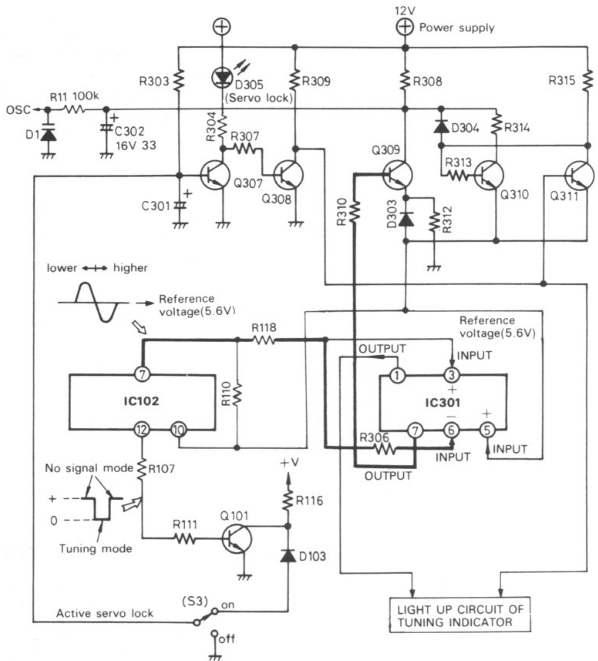
(Active servo lock circuit) Fig. 4
