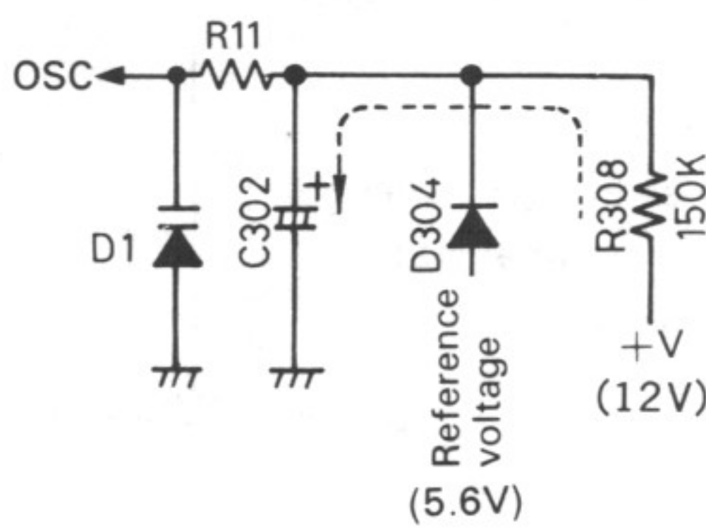
(Exact tuning & deviation to lower frequency) Fig. 6
