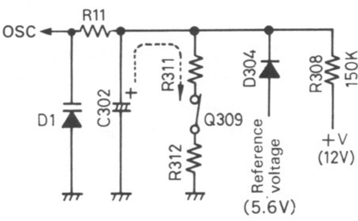
(Deviation to higher frequency) Fig. 7
