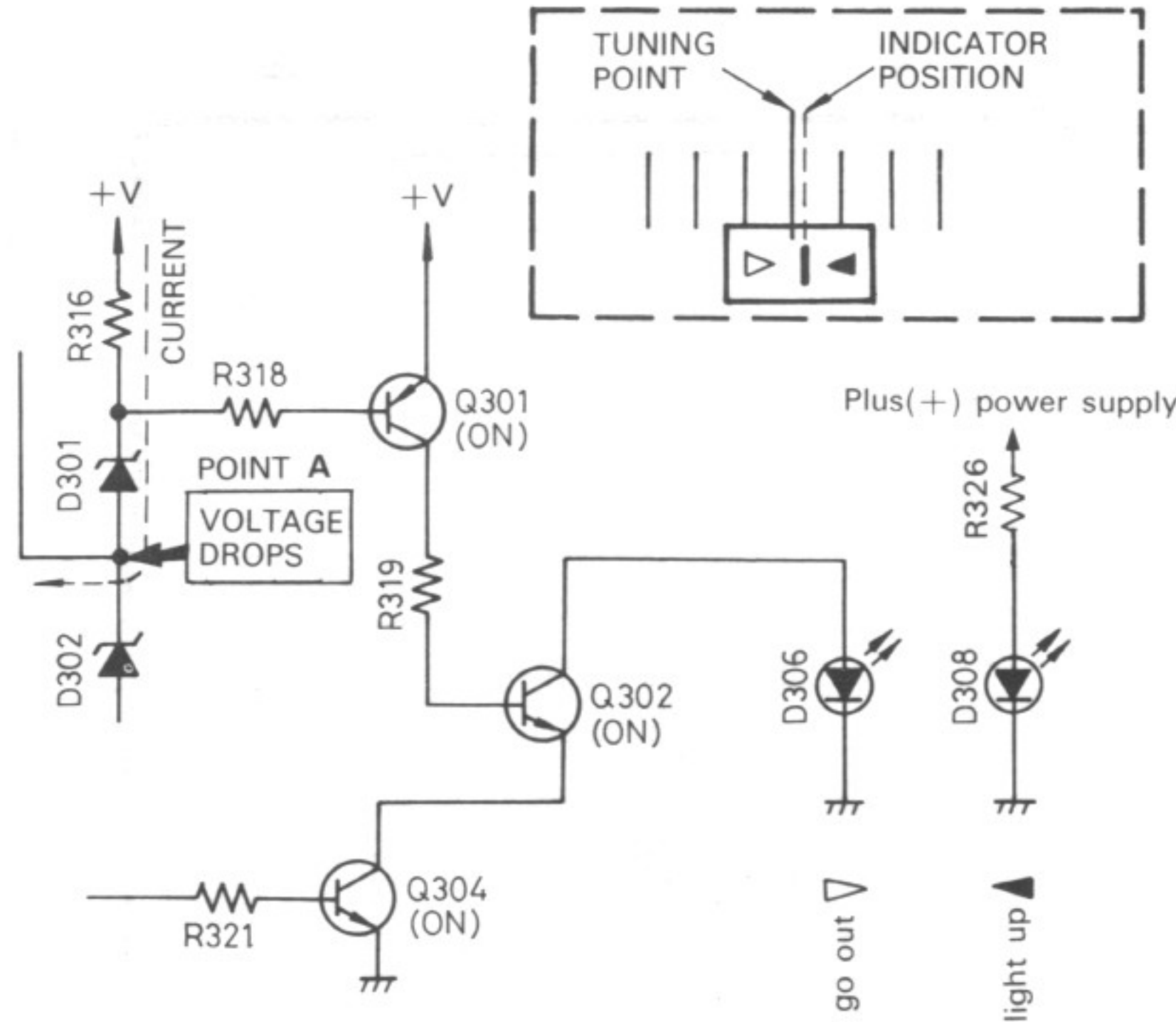
(Deviation to higher frequency) Fig. 10
