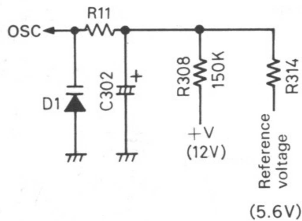
(No signal mode) Fig. 5
